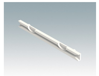
M6490010 Guide-carte, 102 mm PA 6/6 (UL 94 V-0) Fini naturel 101,6x7,5x3,5mm
