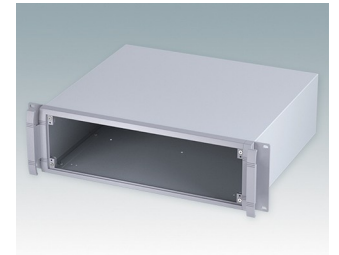
M5619335 UNIMET 19" 3Ux380mm Aluminium Gris clair/gris fenêtre RAL 7035/7040 132,5x482,6x380mm
